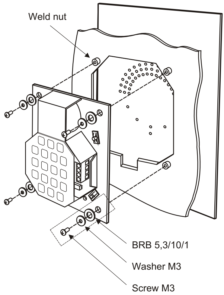
Front panel "arched"
